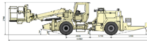
SIDE VIEW Basic machine
