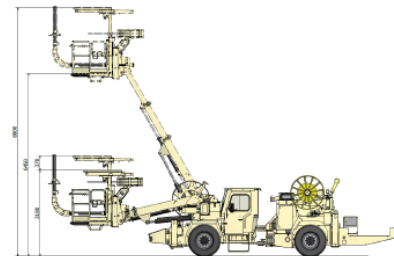
SIDE VIEW Machine with optional and additional equipment
